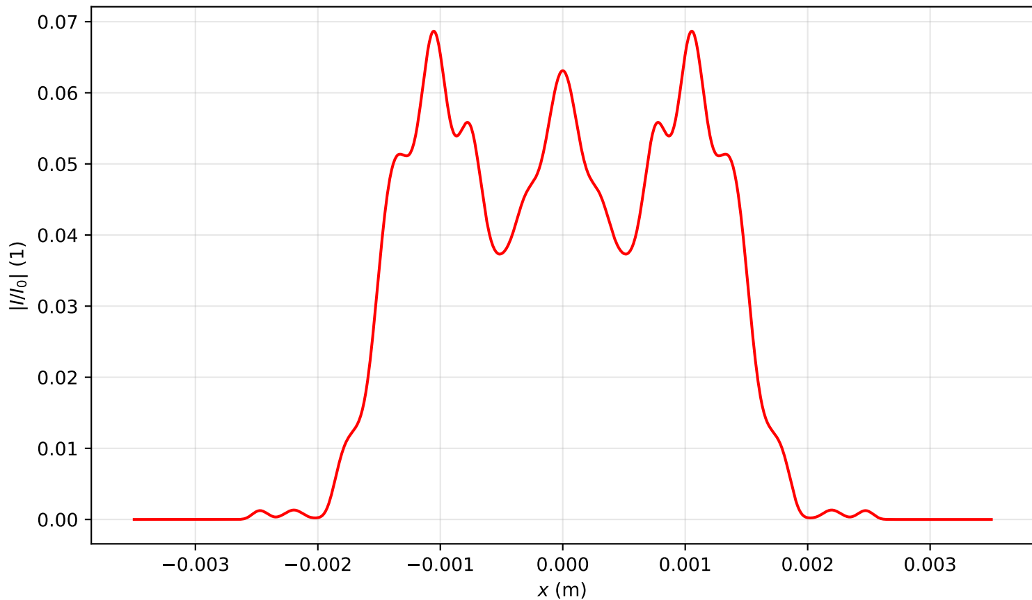
Intensity profile I(x, y = 0, z = 3.105)/I_0 , P_{in}=6.0P_{cr} , artificial time
